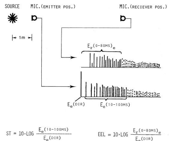
Figure 4: Definitions of ST_{\text{Early}} and EEL
