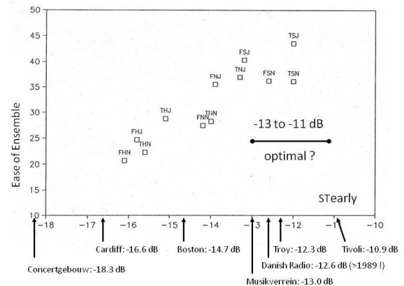
Figure 6: Ease of ensemble versus ST_{\text{Early}} from experiment in the old Danish Radio Concert Hall
