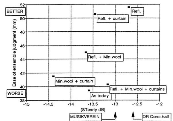
Figure 7: Ease of ensemble versus ST_{\text{Early}} from experiment in the Göteborg Konserthus, Sweden
