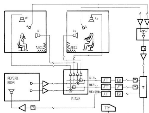
Figure 3. Set up for ensemble experiments at DTU; 1982
